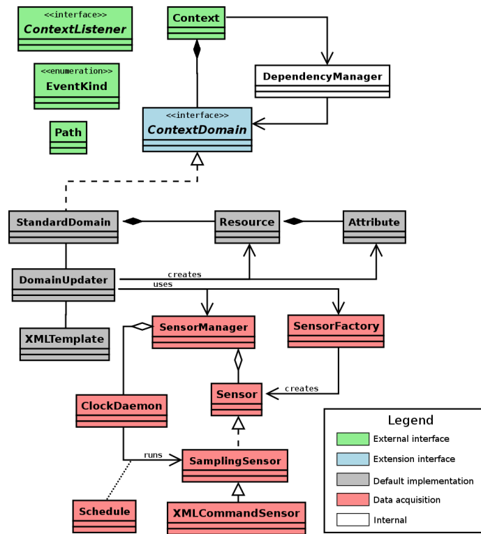
Figure 2: Class diagram of WildCAT internals.
