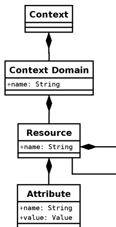
Figure 1: WildCAT’s logical data model.
