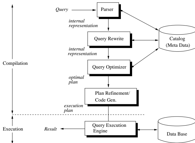
Figure 3: Phases of Query Processing
