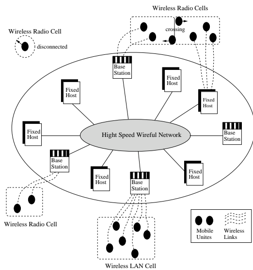
Figure 1: Mobile Computing Architecture
