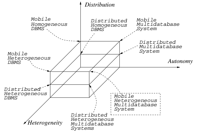
Figure 2: A Classification of Database Systems
